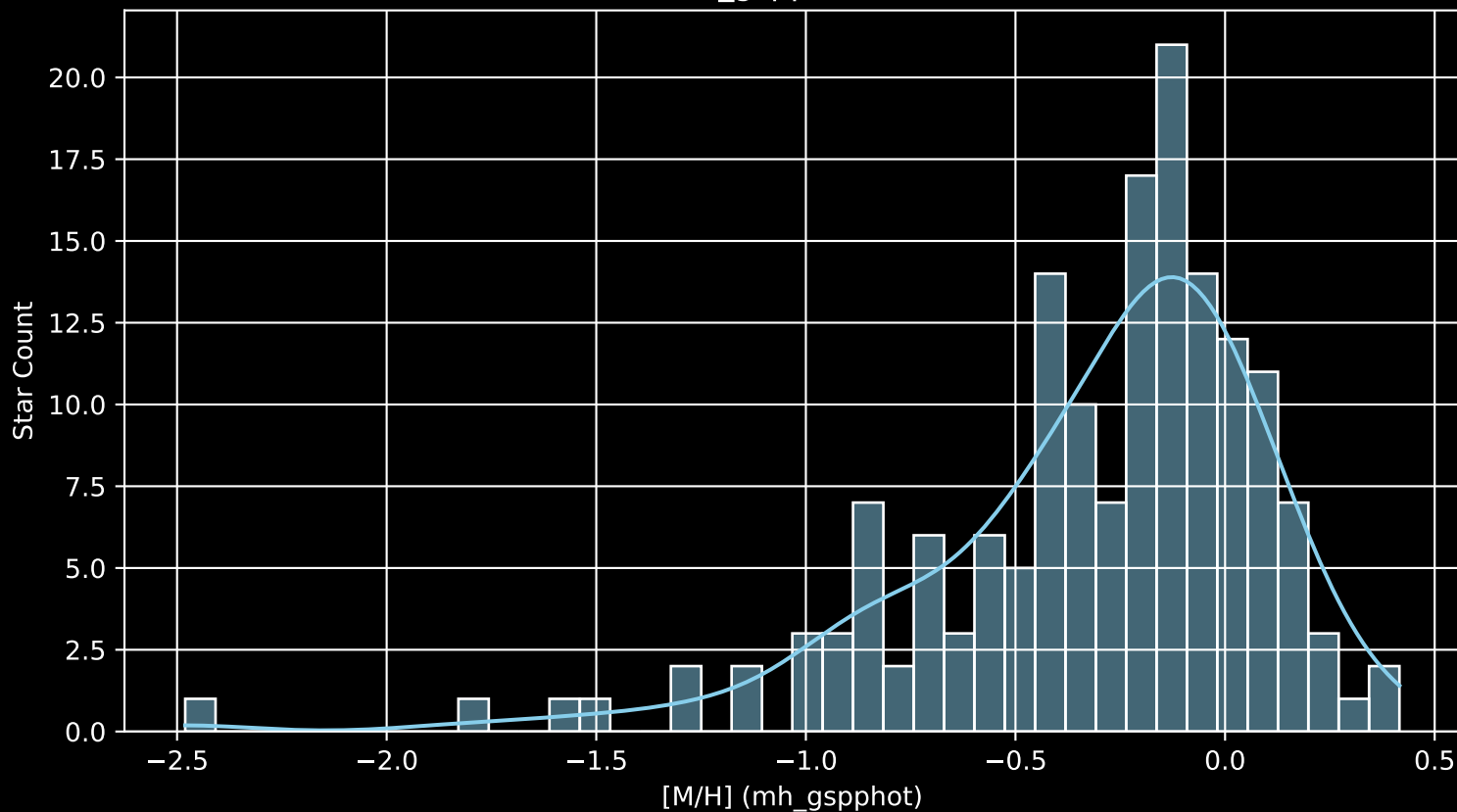
APOGEE DR17 Field: [276-19-O [M/H] (mh_gspphot) (n= 162)
