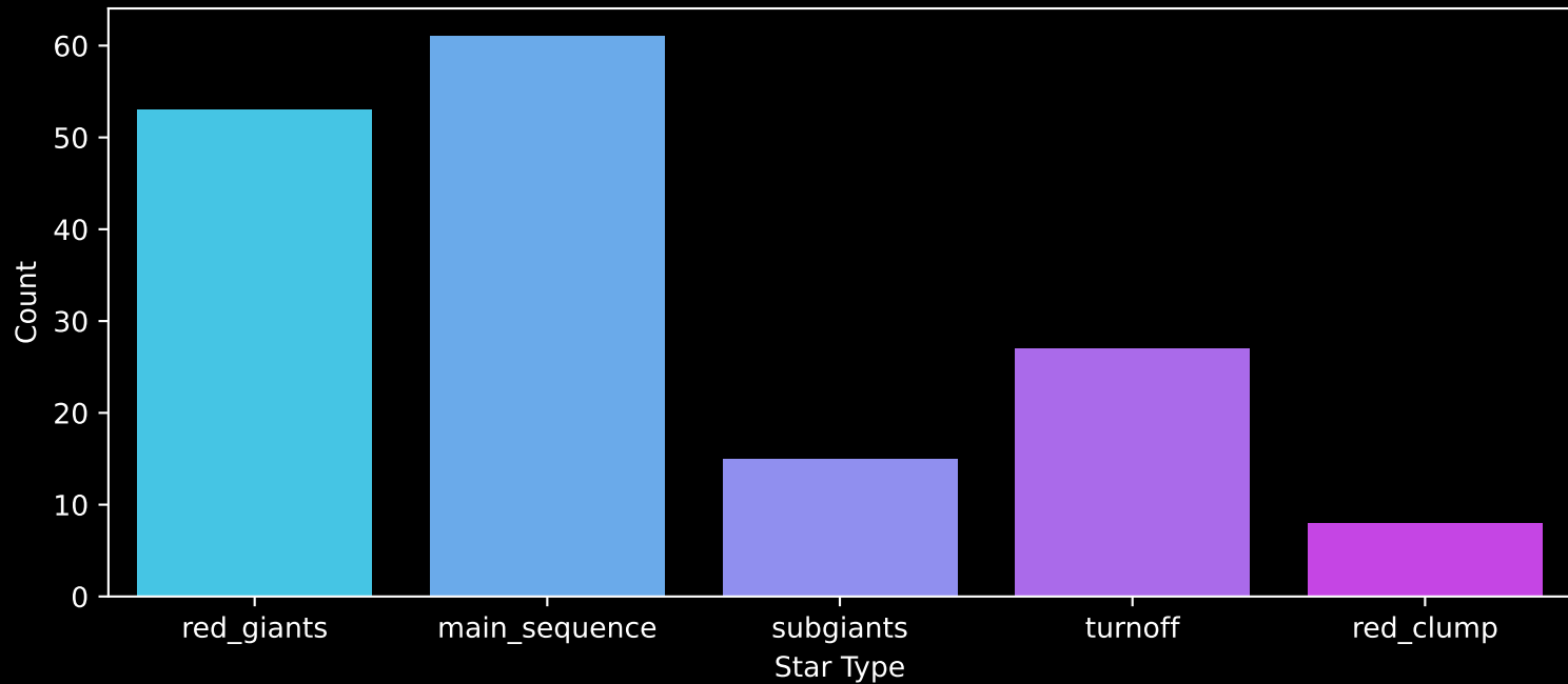
APOGEE DR17 Field: [276-19-O] Count plot of Star Type
