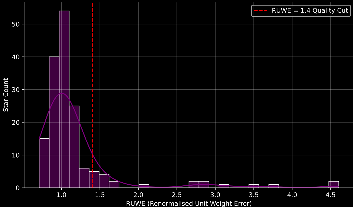
GAPOGEE DR17 Field [276-19-O] RUWE Distribution (n= 161)
