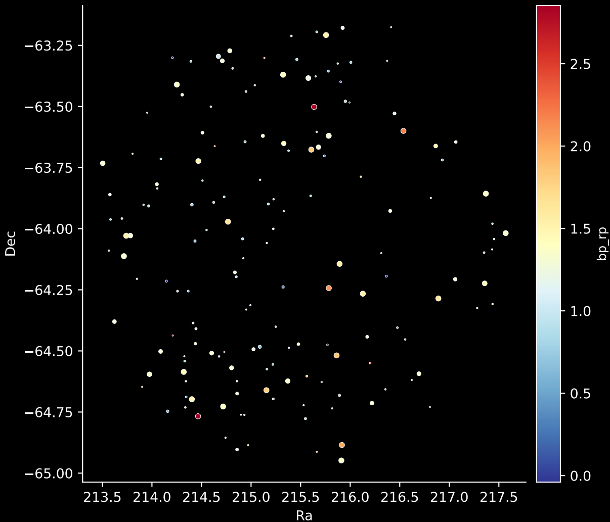
APOGEE DR17 Field: [276-19-O] Stars: 164
