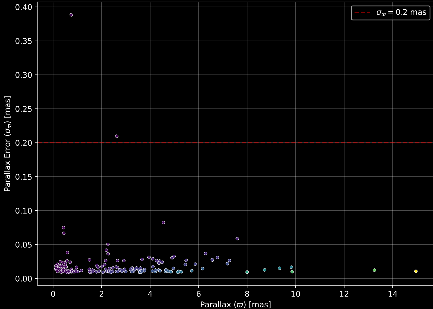
APOGEE DR17 Field: [276-19-O] Parallax Quality (n= 164)
