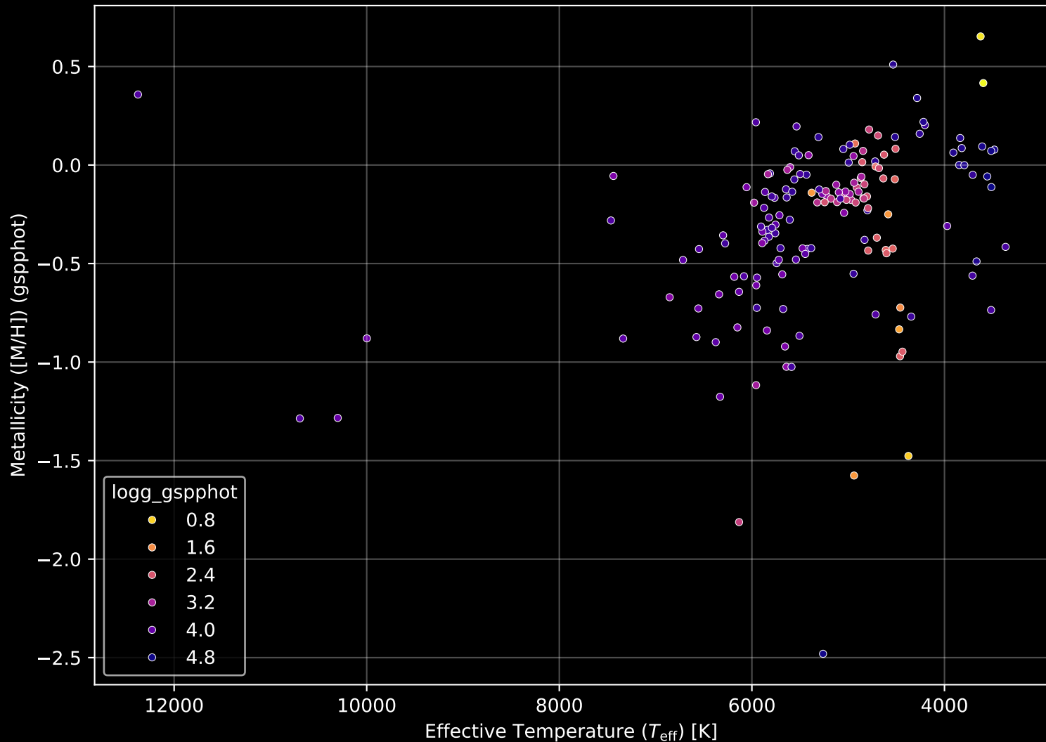
APOGEE DR17 Field: [276-19-O] Stellar Population Parameters (n= 164)
