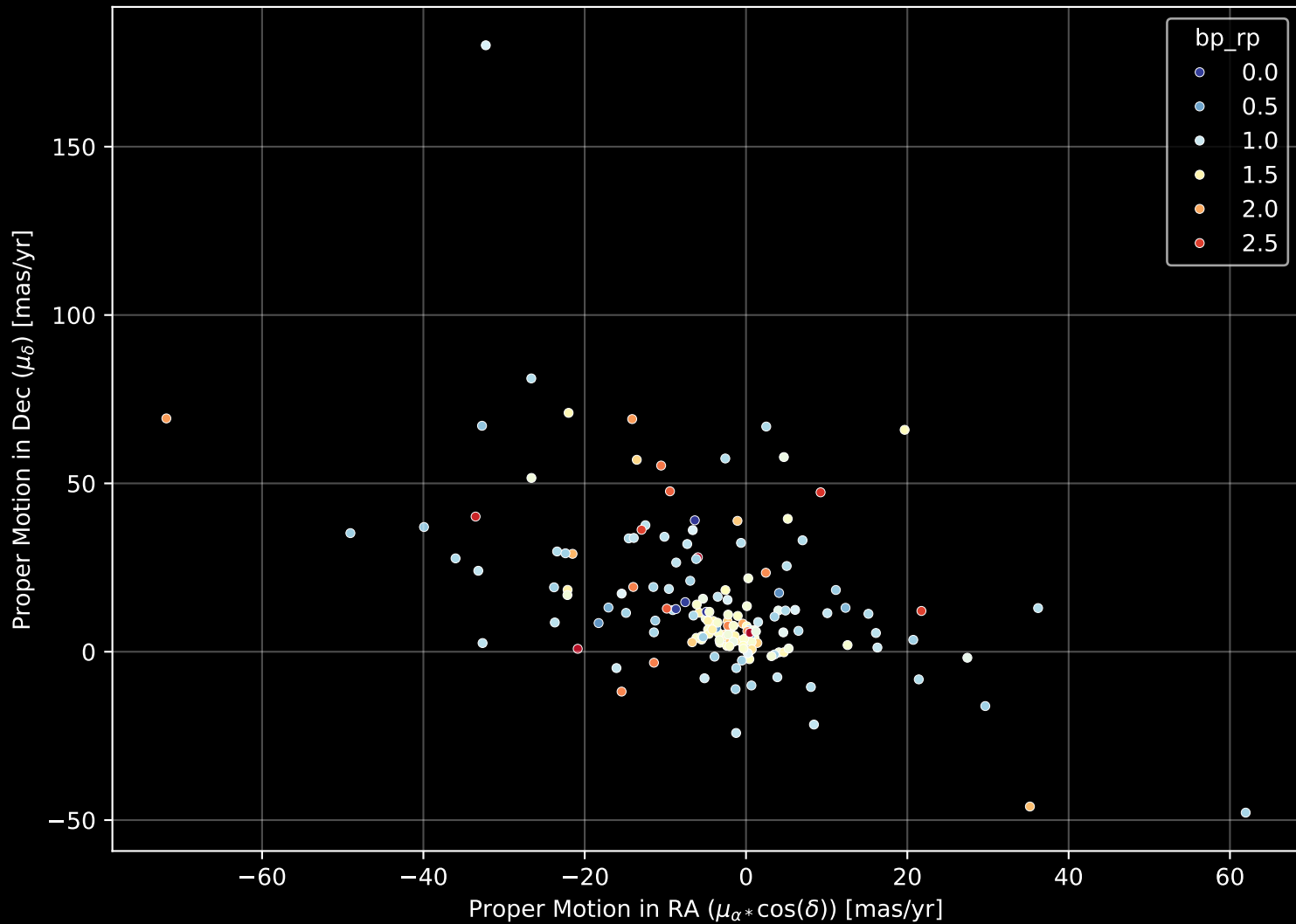
APOGEE DR17 Field: [276-19-O] Proper Motion Diagram (n= 164)
